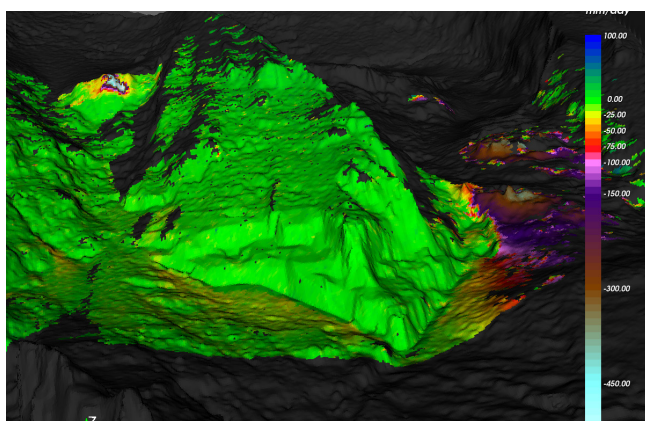
Figure 2: Projection onto digital elevation model: The data of the interferometric radar show increased velocity on the right margin of the glacier.
