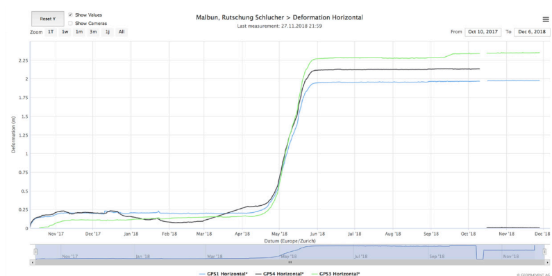
GNSS-station landslide Schlucher (Malbun), Liechtenstein
